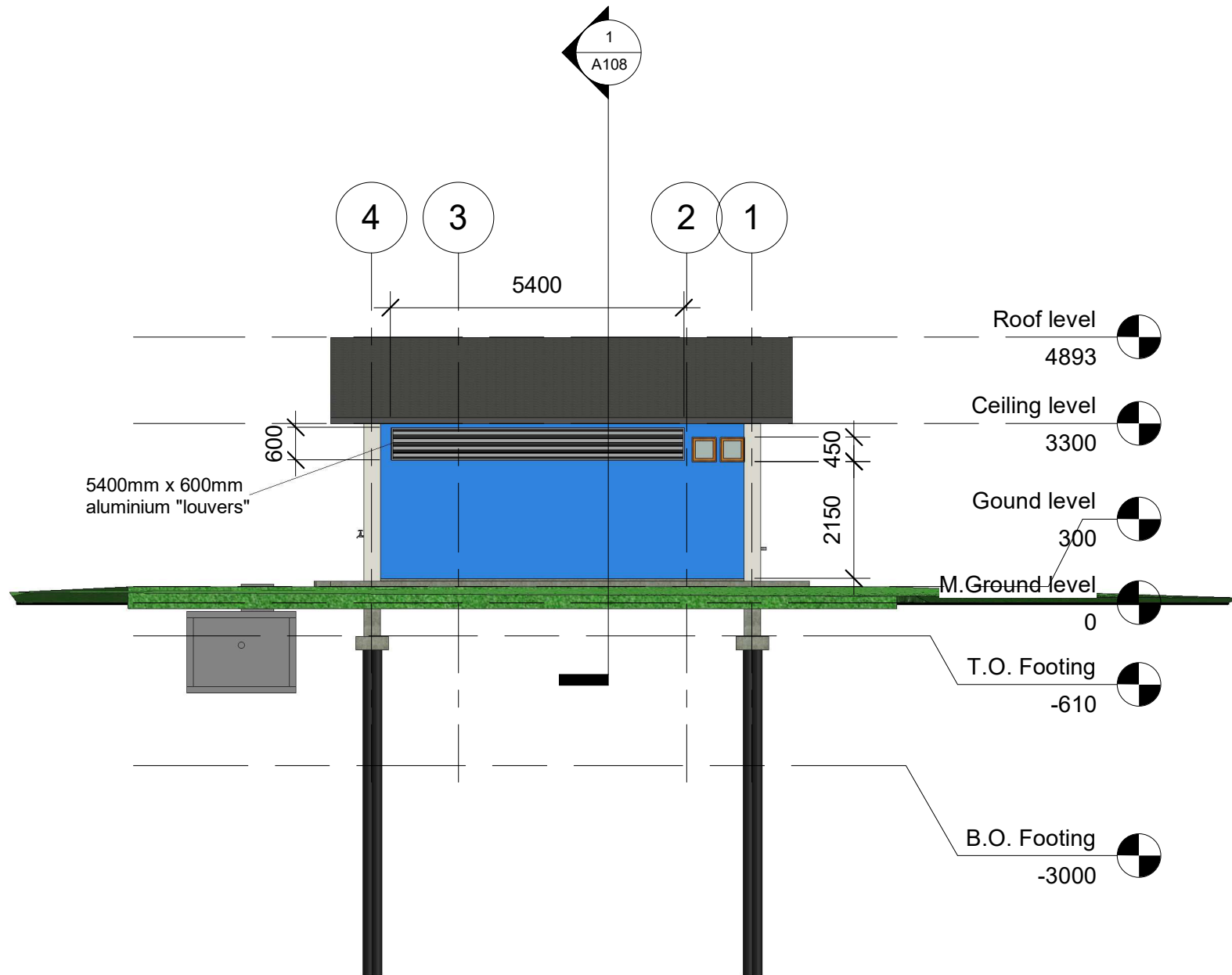
1 Rear Elevation 1 : 100
