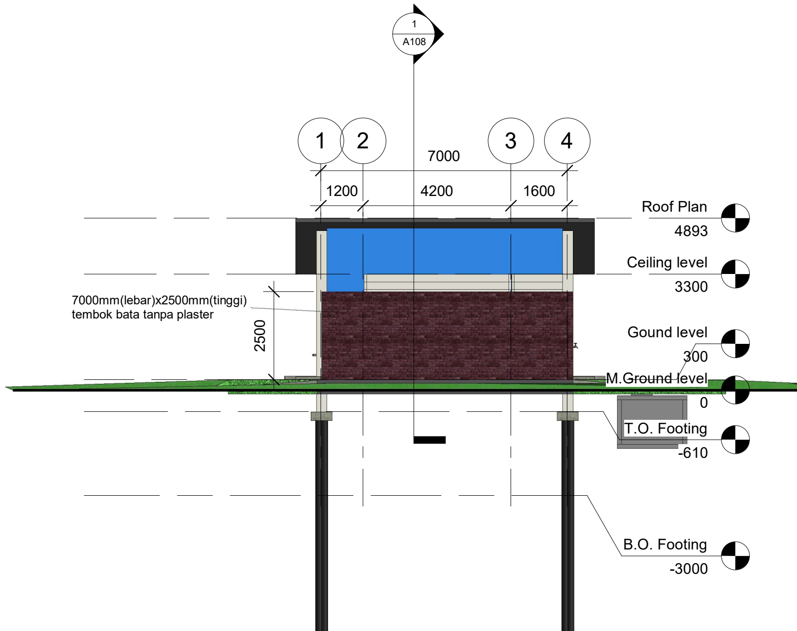
1 Front Elevation 1 : 100
