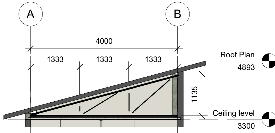
2 Roof Section B-B 1 : 50
