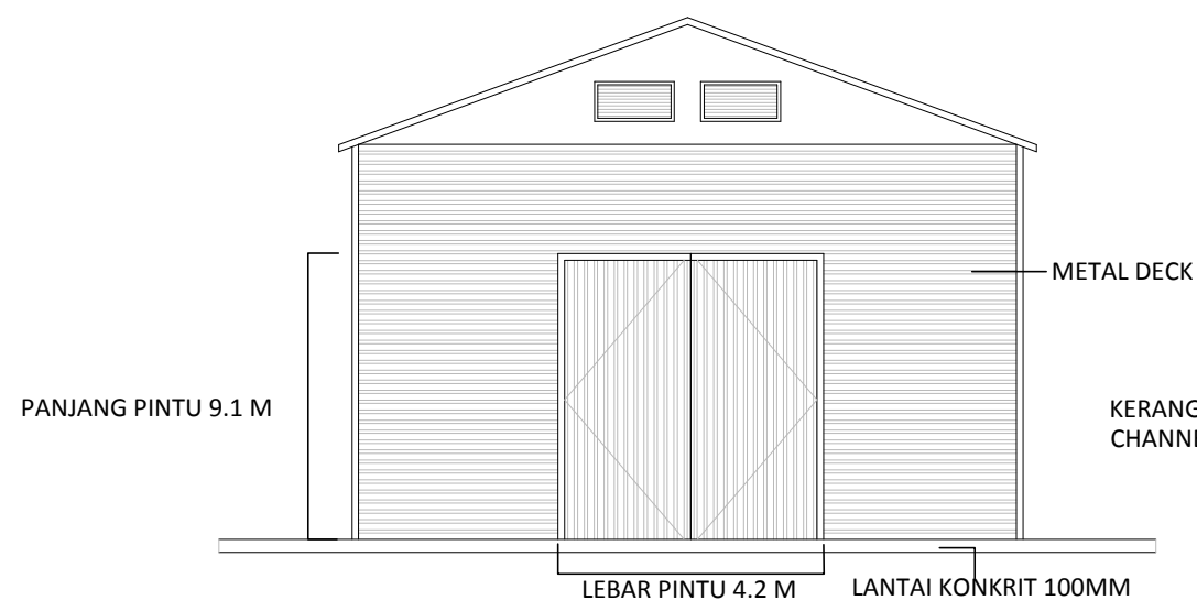
PANDANGAN HADAPAN
