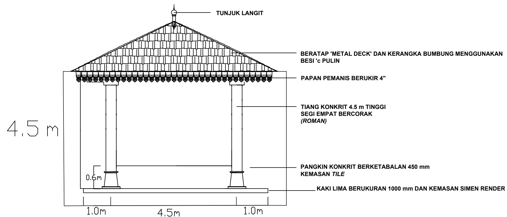
PANDANGAN HADAPAN
